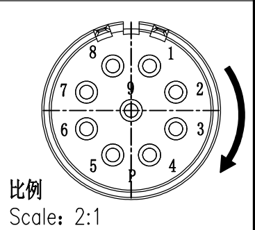
针位排布图 Contact arrangement
