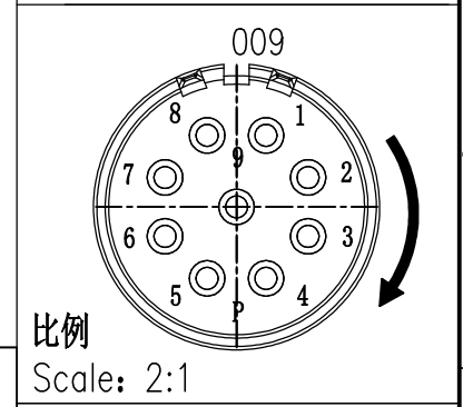
针位排布图 Contact arrangement
