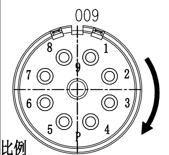
针位排布图 Contact arrangement
