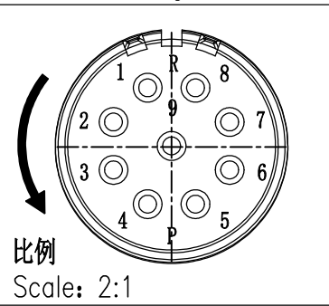
针位排布图 Contact arrangement
