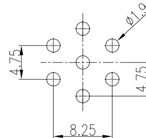
PCB孔细节 PCB layout
