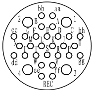
针位排布图 Contact arrangement
