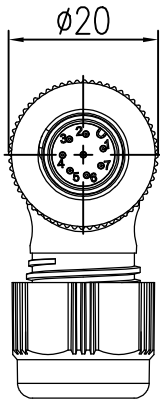
针位排布图 Contact arrangement
