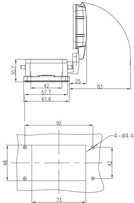
面板开孔图 panel cut out
